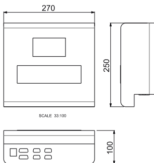
Controller G130/230i
