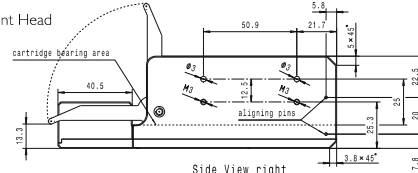
Low Profile Print Head
