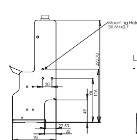
Standard Print Head
