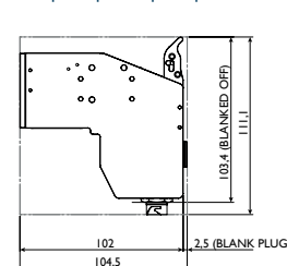
Compacte printkop – topconnector
