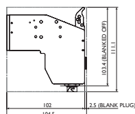
Compact printhead - Top connector
