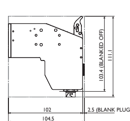
Compact printhead – Top connector
