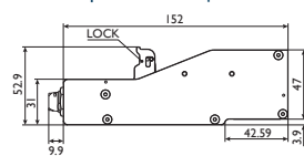
Standard printhead – Top connector
