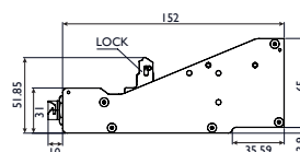
EXT printhead – Top connector
