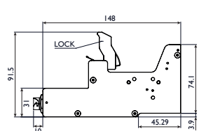
OPT printhead – Top connector
