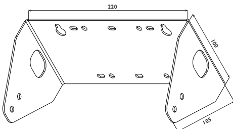
Printer bracket
